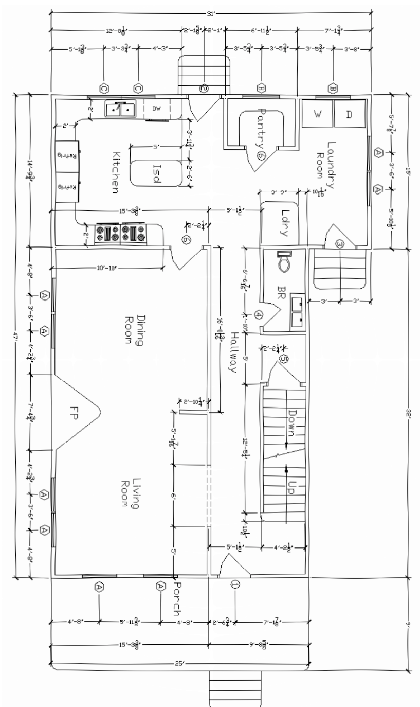
Figure E.1 – The First Floor Plan
